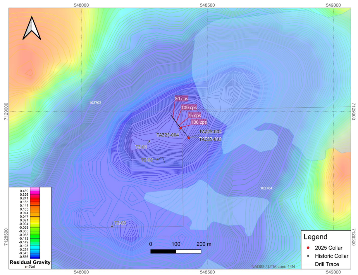
Figure 8: Tarzan target area showing residual gravity and 2025 drill holes.
