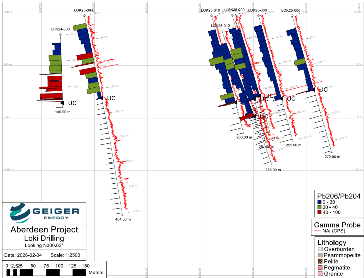
Figure 5: NNE-SSW long section through the Loki area showing Pb^{206}/Pb^{204} ratios. Note extreme anomalies to south in LOK24-003 and LOK25-004.
