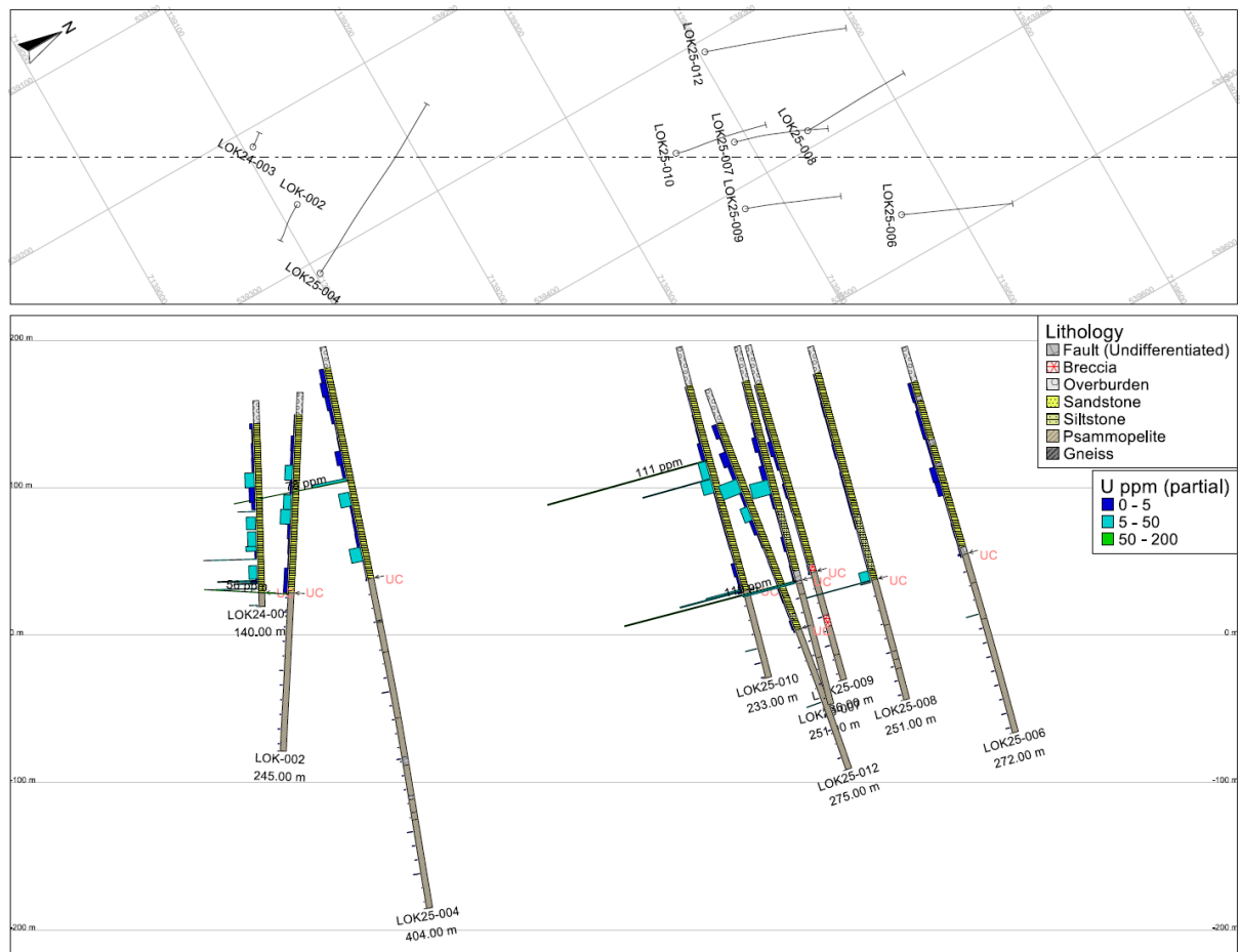
Figure 3: NNE-SSW long section showing drill holes in the Loki area with radioactivity.
