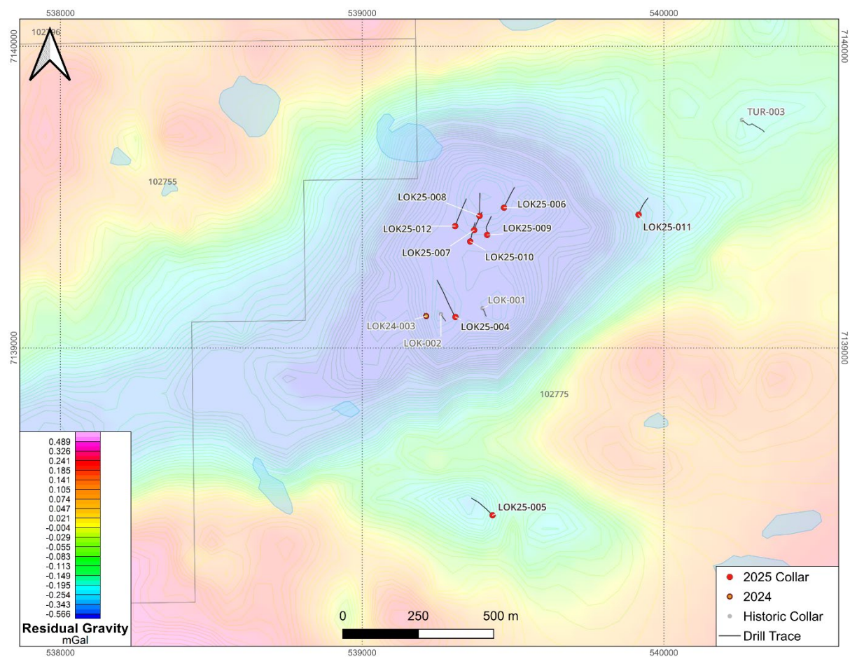
Figure 2: NE part of the Loki target area showing residual gravity and 2025 drill holes and traces.
